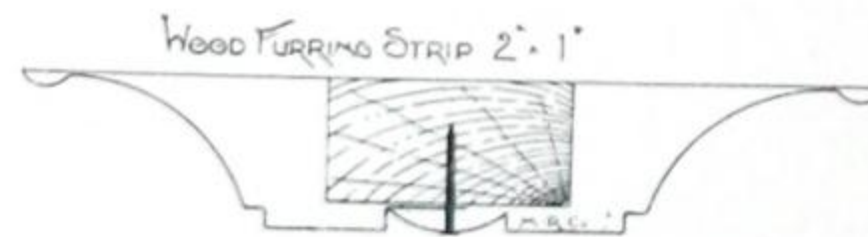
Section of Joint on Plate No. 479.
